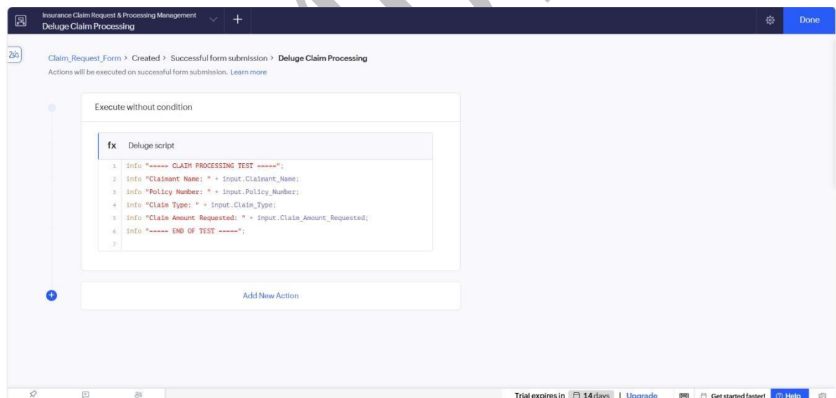
Fig 7: Saved Deluge script inside the workflow
