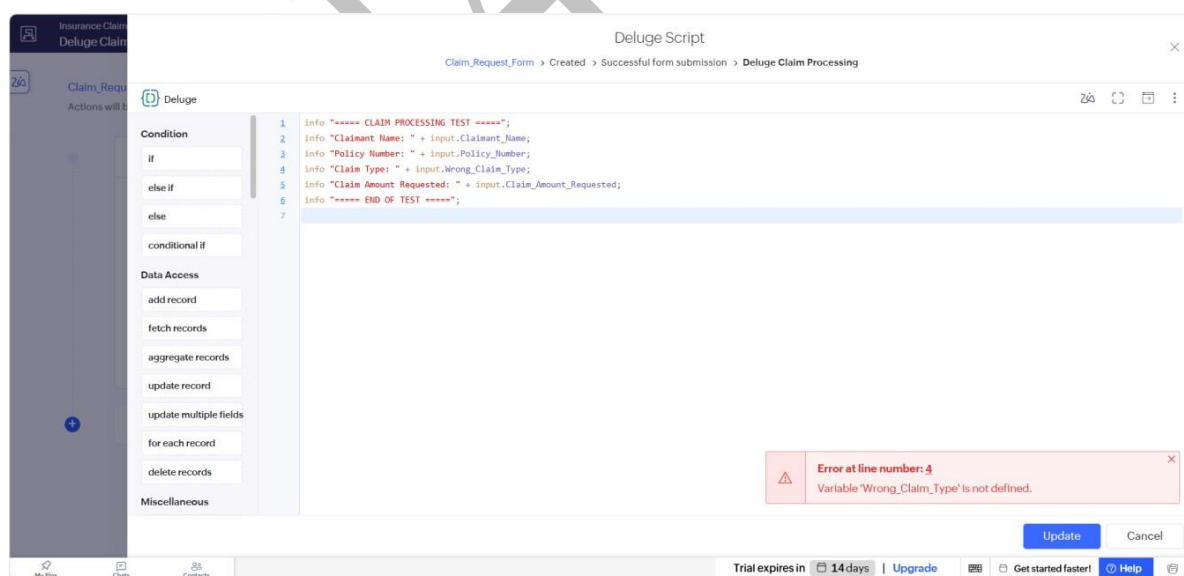
Fig 8: Error message for an undefined variable on line 4
